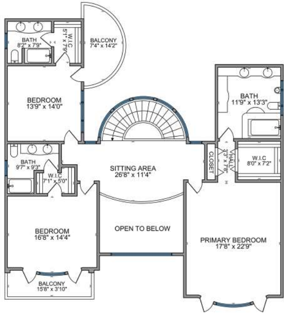
Upper Floor - 2010 SQ. FT Ceiling height - 8'6"
