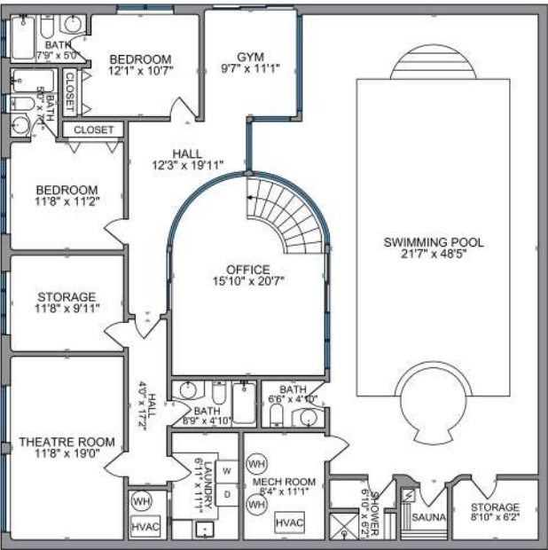
Lower Floor - 1955 SQ. FT Ceiling height - 8'6"
